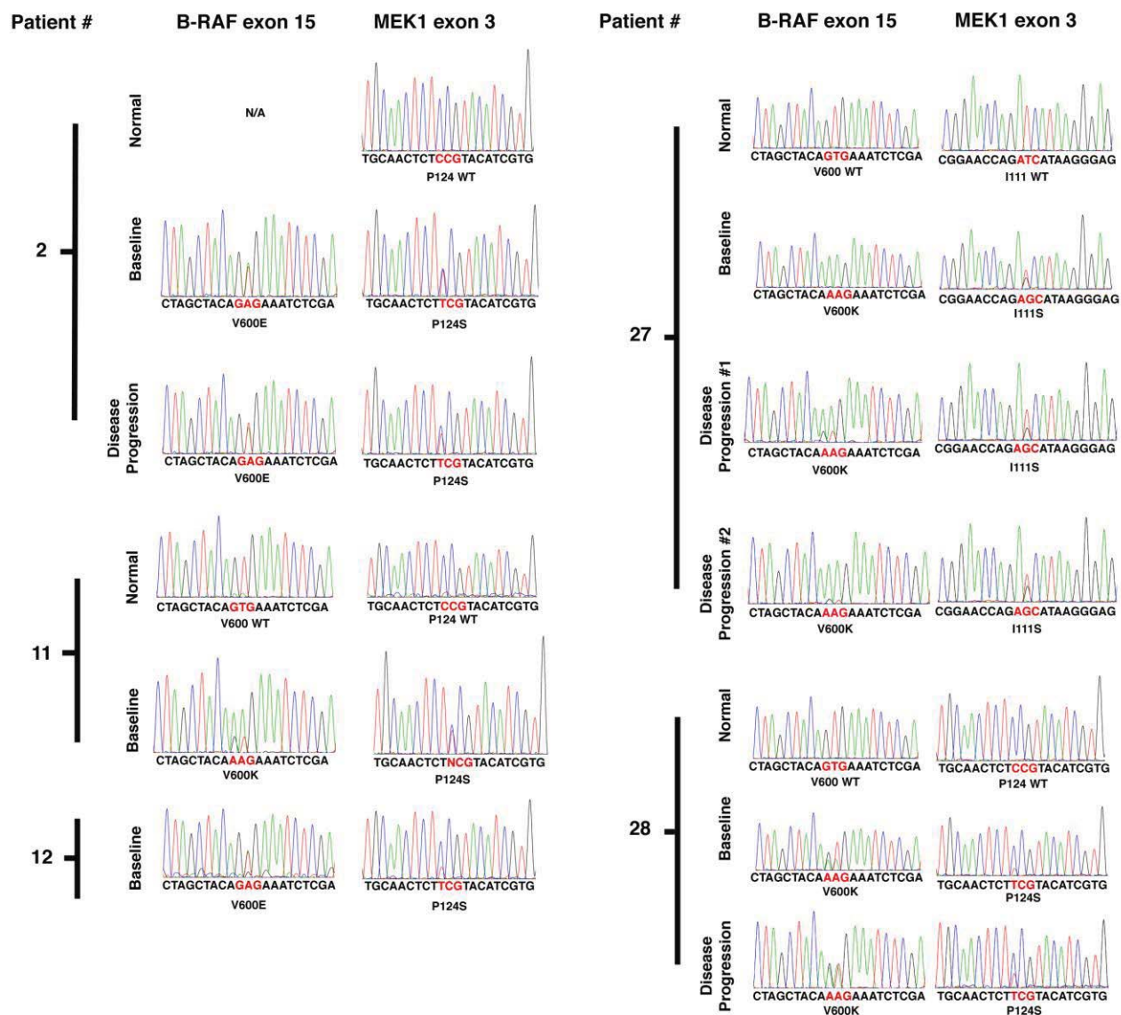
Supplementary Figure. S1. Patient tissues harboring concurrent and somatic B-Raf and MEK1 mutations. Chromatograms showing B-Raf exon 15 at V600 codon and MEK1 exon 3 at I111 or P124 codons in patient-matched normal tissue, baseline melanomas (prior to B-RaFi therapy), and melanomas on disease progression (i.e. at acquisition of B-RaFi resistance). Specific codons in red; N/A, not available.
